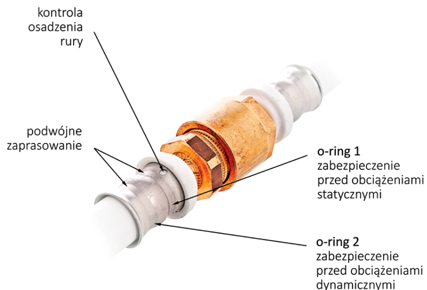
Rys. 1. System HERZ PipeFix
